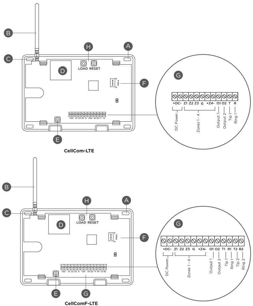
New CellCom PCB PC-0207
