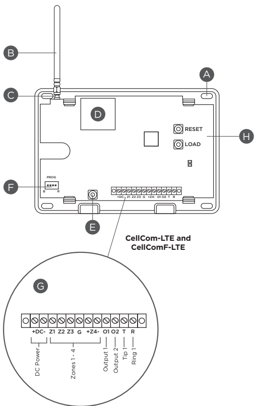
Previous CellCom PCB PC-0163
